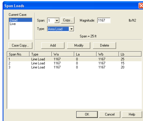
Figure 4-49 Defining Area Load on Span
