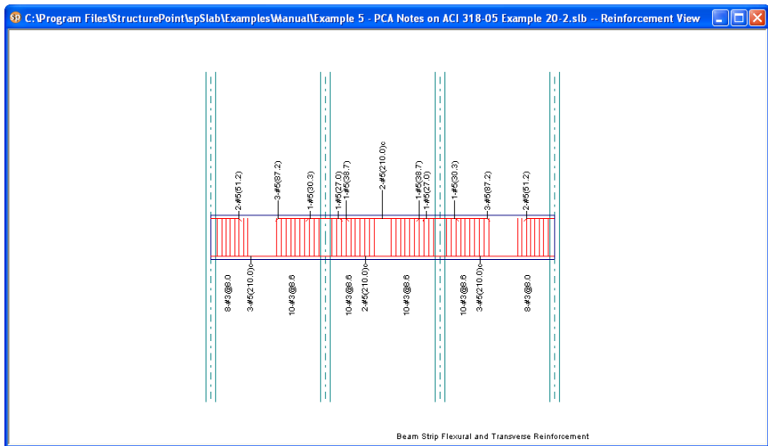
Figure 4-85 View Reinforcement
