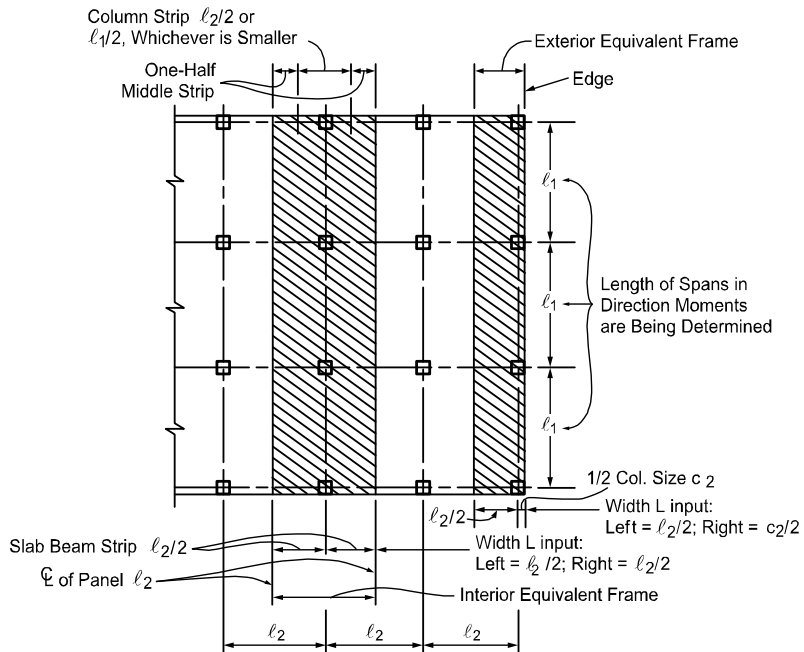
Figure 2-5 Design strips
